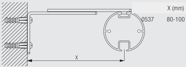
0537 Adjustable bracket
